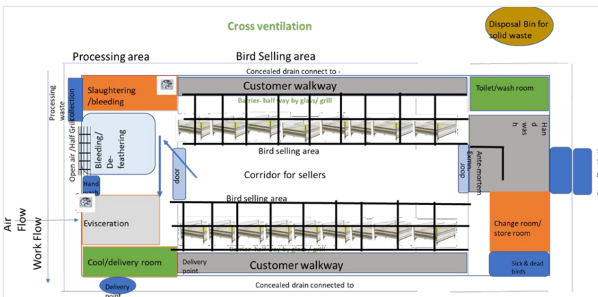
Figure 20. Design 3: Proposed layout for newly constructed LBMs
